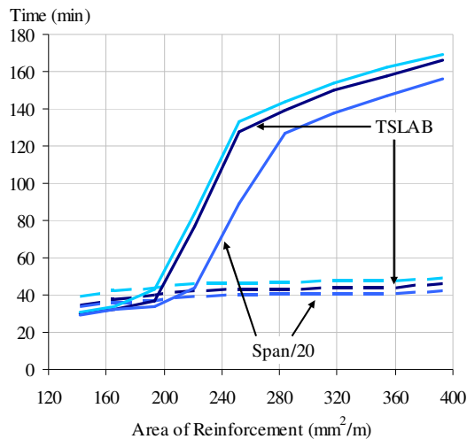
Fig. 14: Comparison of Bailey-BRE and Vulcan Failure times for 9m x 6m slab panel
