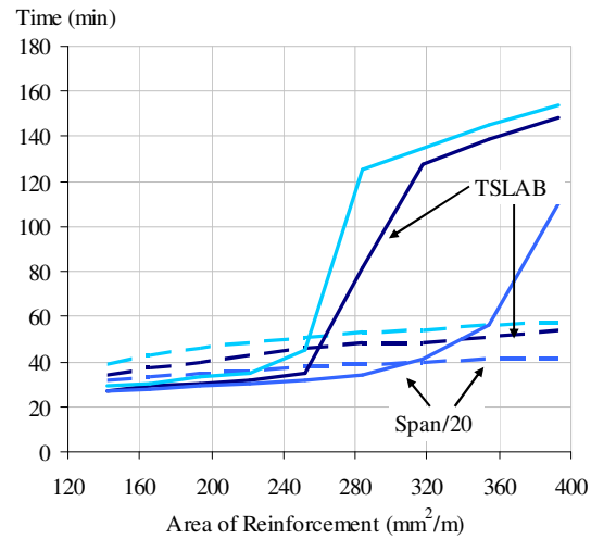
Fig. 15: Comparison of Bailey-BRE and Vulcan Failure times for 9m x 12m slab panel
