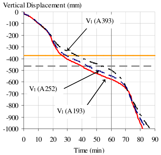
Fig. 8: Reinforcement ratio comparison
