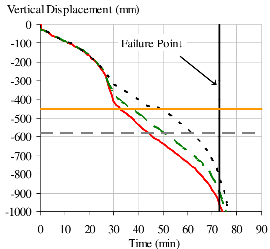
Fig. 13: Plastic failure of 9m x 9m slab panel
