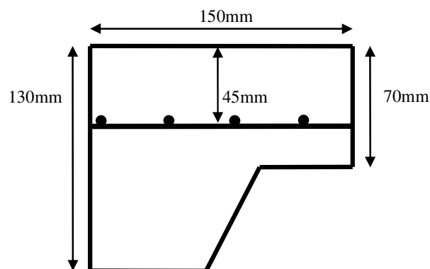
Fig. 3: Concrete slab cross-section
