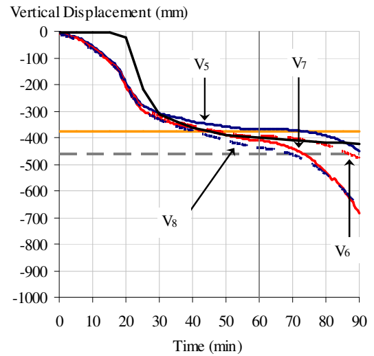
Fig. 10: Influence of Rotational restraint
