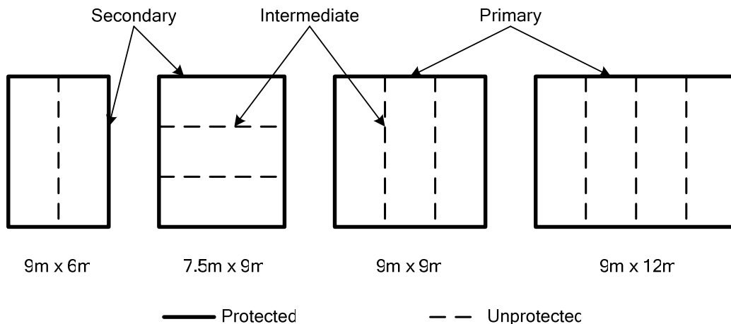
Fig. 2: Slab Panel Sizes
