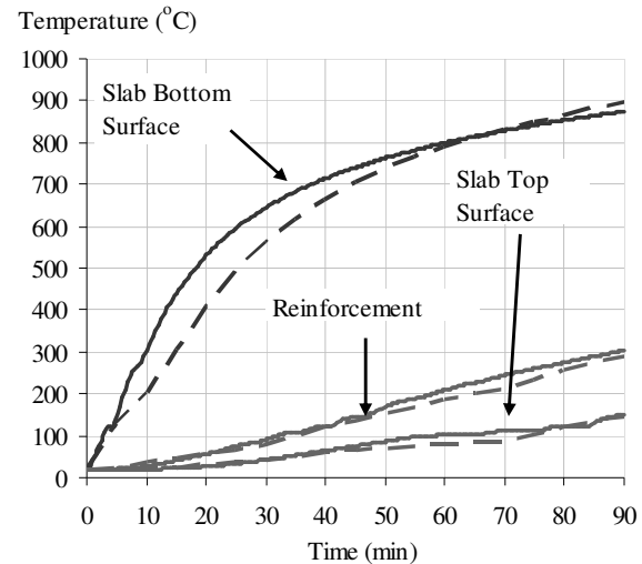
Fig. 4b: Comparison of thermal distribution through the depth of the 1D slab profile
