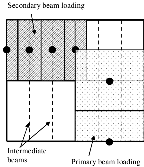
Fig. 11a Load distribution – Type 1 failure
